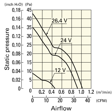
9LG0824F4001 With pulse sensor
