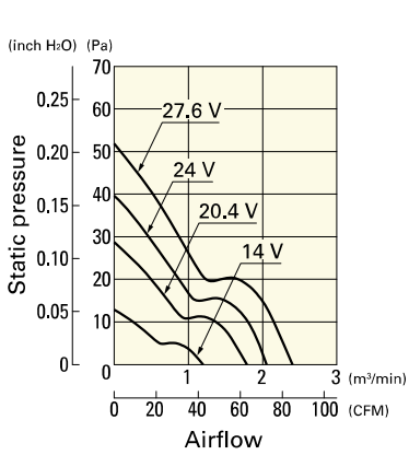
9WP1224M101 With pulse sensor
