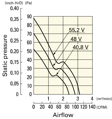
9WP1248H101 With pulse sensor
