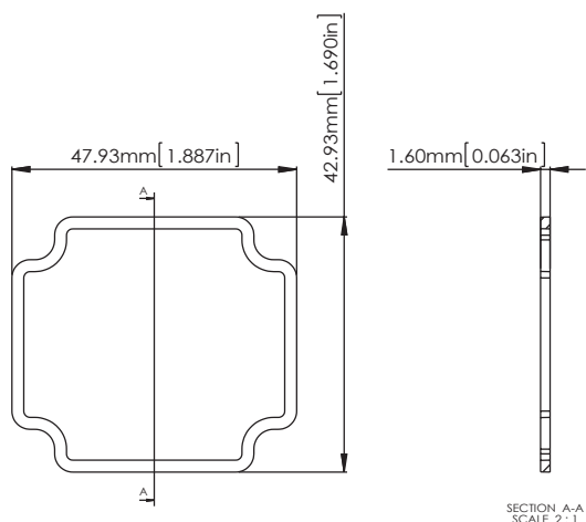
G101-Seal
