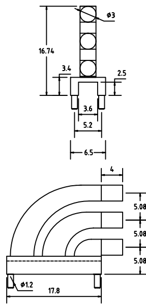
Dimensions in mm (typical)
