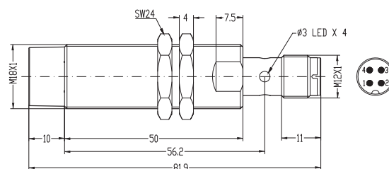
Fig. 13 Long body, non-flush version, plug
