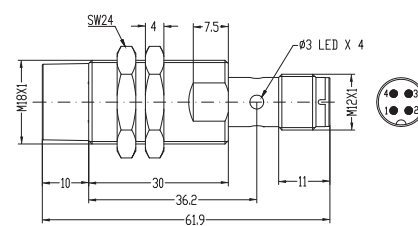
Fig. 9 Short body, non-flush version, plug
