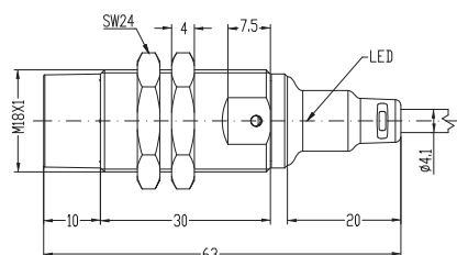
Fig. 7 Short body, non-flush version, cable
