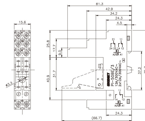
Appearance illustration
