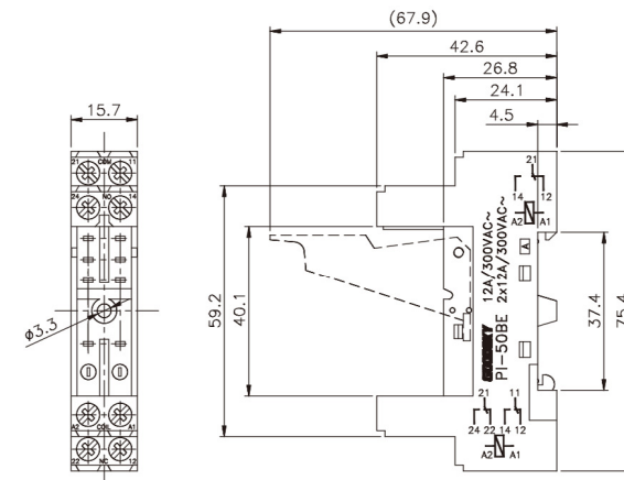
Appearance illustration
