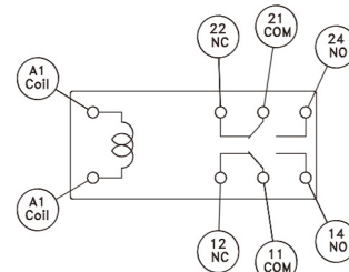
Terminal illustration
