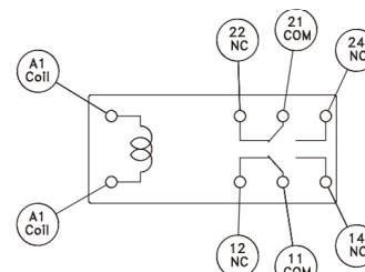
Terminal illustration
