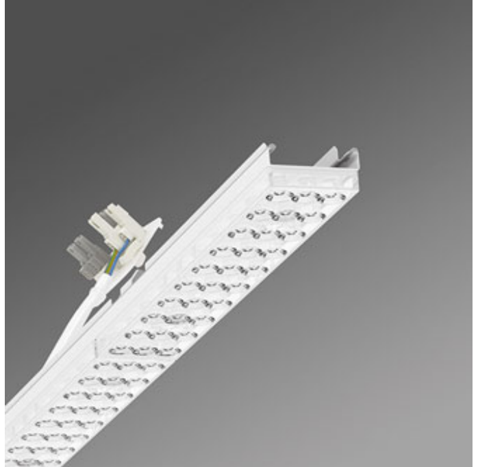
SDGVOTB LED 8000lm 840 - vw - DALI - 18530306650
