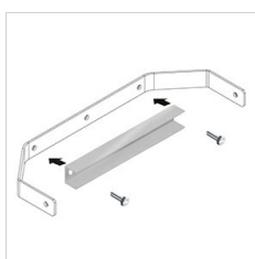
14461104 GUELL 3 strengthening bracket. Suitable for one floodlight single point fixing M10 screw in centre of the bracket Stainless steel
