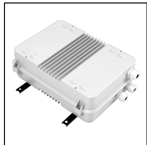
14474094 Drivers box 900 W - 1.4A - 3CH - 220-240 V 50/60 Hz ■ GR-94 / Metallic grey
