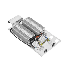
3105741 Drivers unit 470 W - 1.1A - 2CH - 1-10 V - - 380-415V 50/60 Hz
