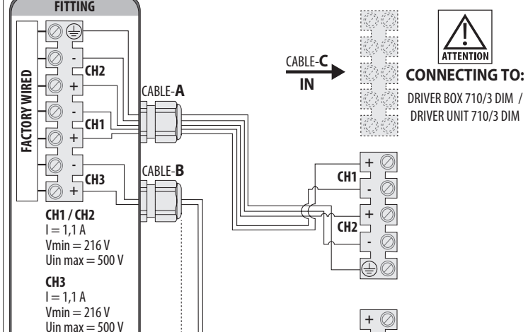
SQUARE PRO GLASS 710/3 (1.1 A V=216 V U in max=500 V) + DRIVER 710/3 DIM : 710 W
