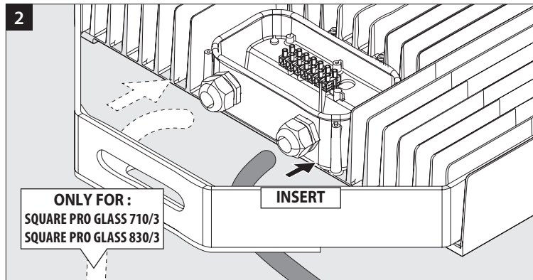
SQUARE PRO GLASS 710/3 (1.1 A V=216 V U in max=500 V) + DRIVER 710/3 DIM : 710 W
