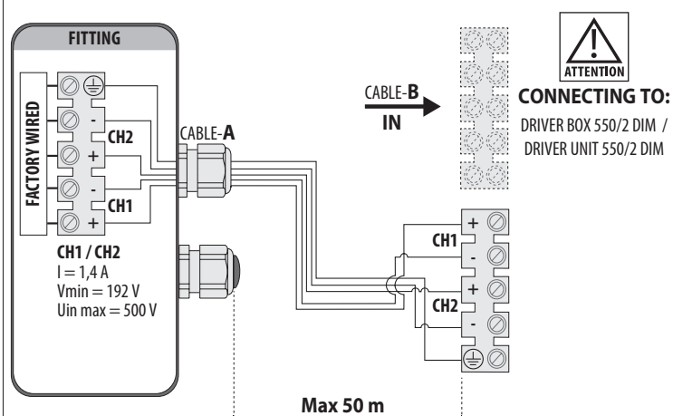
SQUARE PRO GLASS 550/2 (1.4 A V=192 V U in max=500 V) + DRIVER 550/2 DIM : 550 W
