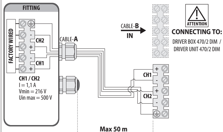
SQUARE PRO GLASS 470/2 (1.1 A V=216 V U in max=500 V) + DRIVER 470/2 DIM : 470 W
