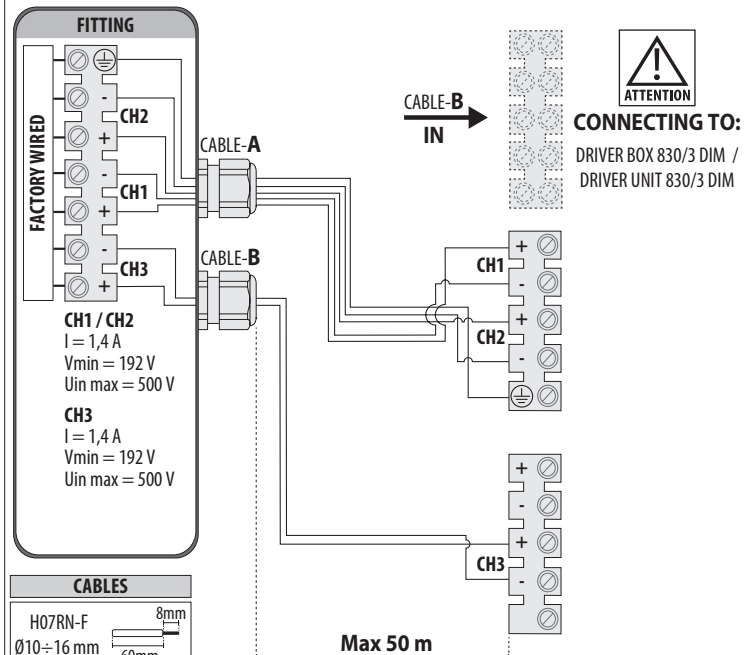
SQUARE PRO GLASS 830/3 (1.4 A V=192 V U in max=500 V) + DRIVER 830/3 DIM : 830 W
